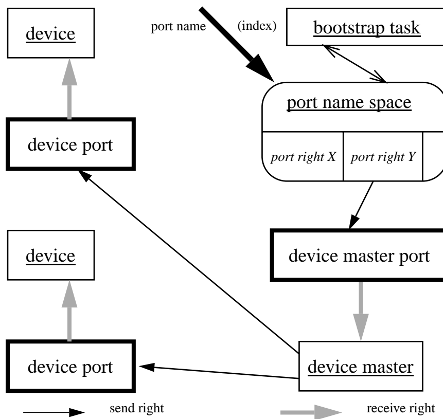
FIGURE 12 Device Structures
